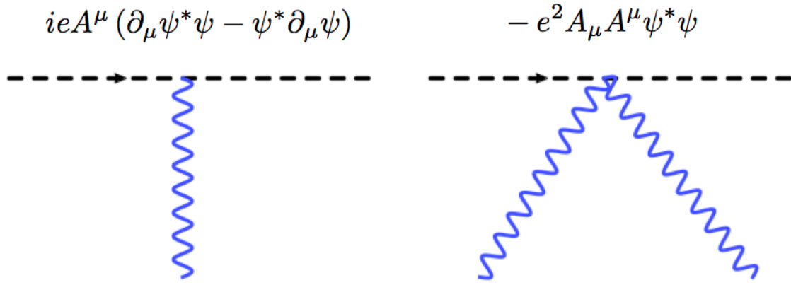
Figure 12. The photon-scalar interaction vertices in scalar QED, see Eq. (3.75) and the corresponding discussion in the text more more details.
