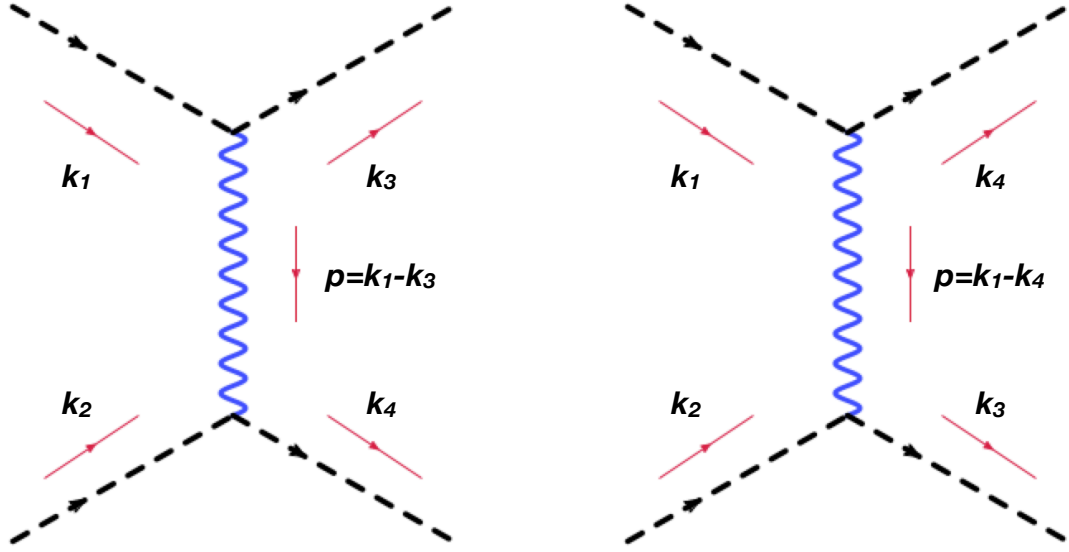
Figure 14. Feynman diagrams relevant for the calculation of Moeller scattering, e^-e^- \rightarrow e^-e^- , at tree level in scalar QED. See text for more details.
