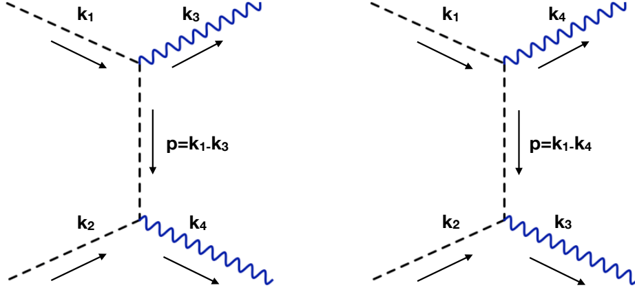
Figure 15. Feynman diagrams relevant for the calculation of the tree level scattering process e^- + e^- \rightarrow \gamma + \gamma in scalar QED. See text for more details.
