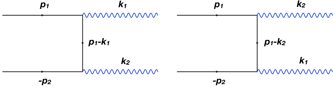
Figure 20. The Feynman diagram for the process of electron-positron annihilation into a photon pair in spinor QED, corresponding to t -channel and u -channel scattering respectively.
