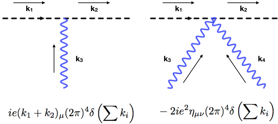
Figure 13. The Feynman rules for the interaction vertices in scalar QED.
