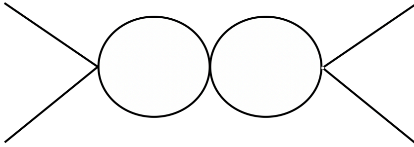
Figure 10. Feynman diagram corresponding to a two-loop calculation to the \phi\phi \rightarrow \phi\phi scattering amplitude in \lambda\phi^4 theory.
