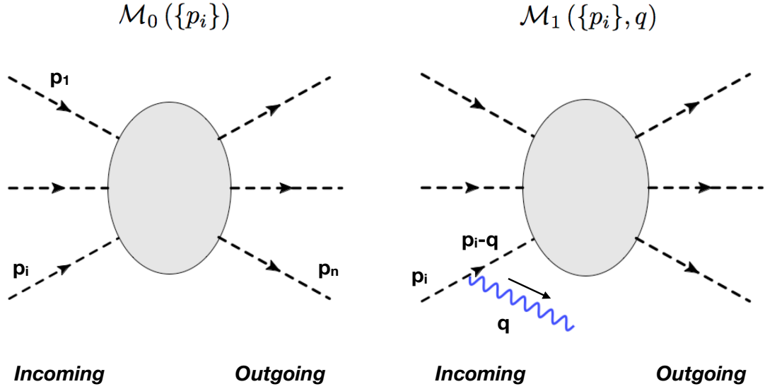
Figure 18. Left plot: a generic scattering amplitude in scalar QED, denoted by \mathcal{M}(\{p_i\}) , consisting of a number of incoming and outgoing (scalar) electrons or positrons. Right plot: the same diagram, now with an outgoing photon with momentum q attached to the incoming scalar leg i . In this case the full scattering amplitude is denoted by \mathcal{M}(\{p_i\}, q) , see text for more details.
