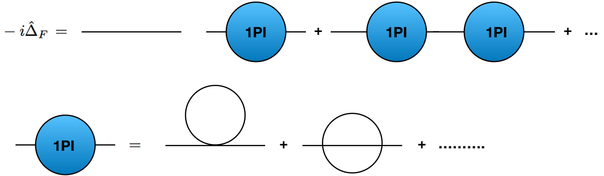
Figure 7. The perturbative expansion of the interacting propagator \Delta_F in Fig. 6 can also be organized in terms of diagrams with different number of 1PI diagrams.
