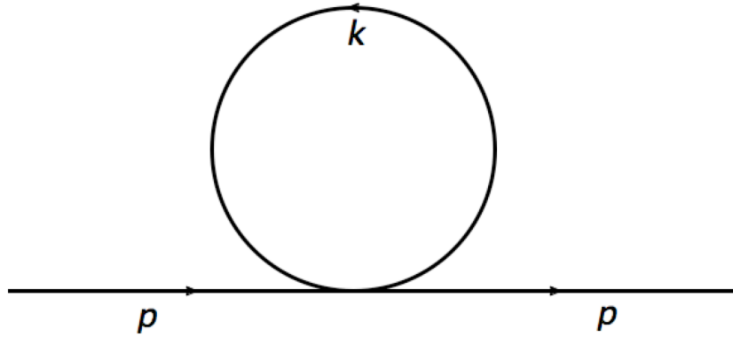
Figure 3. One of the loop diagrams that arise in calculations using \lambda\phi^4 theory beyond the Born approximation, with k^\mu being the four-momentum running in the loop.
