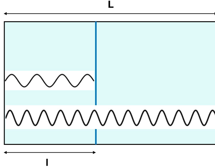
Figure 4. Setup for the Casimir effect. A box of length L contains a perfectly reflective plate at a distance l from one side of the box. We impose Dirichlet boundary conditions both at the sides of the box, \phi(x=0) = \phi(x=L) = 0 and at the plate \phi(x=l) .
