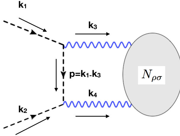
Figure 17. The Feynman diagram for a similar scattering amplitude as that of Fig. 15 but where now the two photons are internal lines (so off-shell) rather than outgoing particles, and where we denote in full generality the rest of the diagram by N^{\rho\sigma} .
