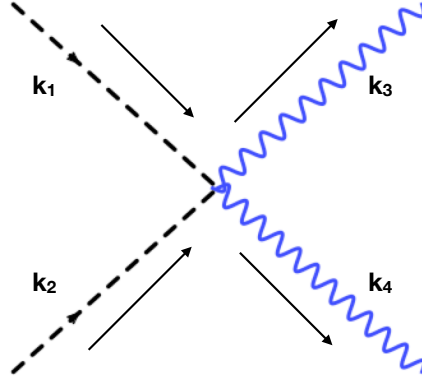
Figure 16. The other Feynman diagram that contributes to the scattering amplitude of the e^-e^- \rightarrow \gamma\gamma in scalar QED at \mathcal{O}(e^2) , in addition to the two diagrams already shown in Fig. 16.
