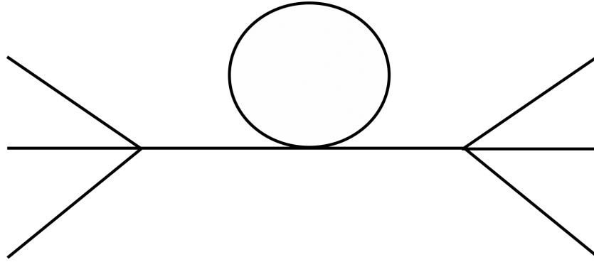
Figure 11. The one-loop correction to the six-point scattering amplitude \mathcal{M}(\phi\phi\phi + \phi\phi\phi) in \lambda\phi^4 theory. Without computing this diagram we can state that it will not contain divergences, since its apparent degree of divergence is D = 4 - E = 4 - 6 = -2 < 0 .
