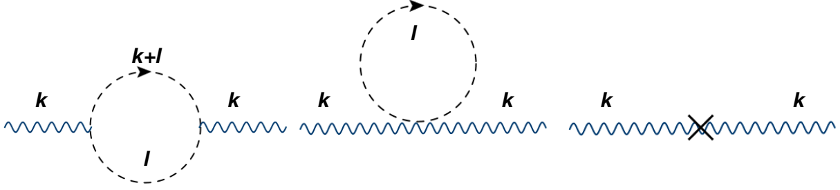
Figure 19. The three Feynman diagrams for the \mathcal{O}(e^2) contributions to the photon self-energy in scalar QED. The last term corresponds to the counterterm associated to the photon propagator being treated as an interaction term.
