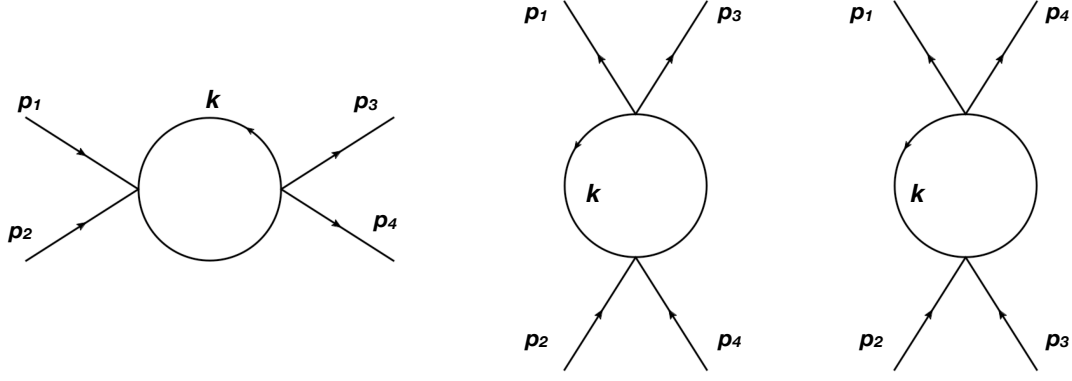
Figure 5. The Feynman diagrams relevant the calculation of the \mathcal{O}(\lambda^2) contribution to the 2 \rightarrow 2 scattering amplitude in \lambda\phi^4 theory. From left to right the topologies correspond to s -channel, t -channel, and u -channel respectively.
