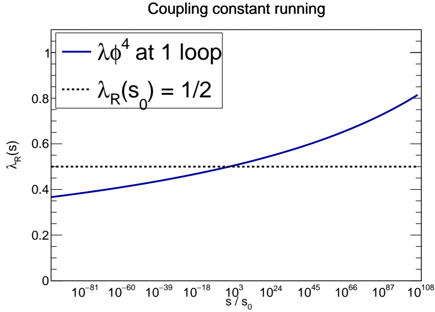
Figure 9. The one-loop running of the renormalized coupling constant \lambda_R(s) in \lambda\phi^4 theory, Eq. (2.101), as a function of the scale ratio s/s_0 . The reference value of the coupling constant has been taken to be \lambda_R(s_0) = 1/2 .
