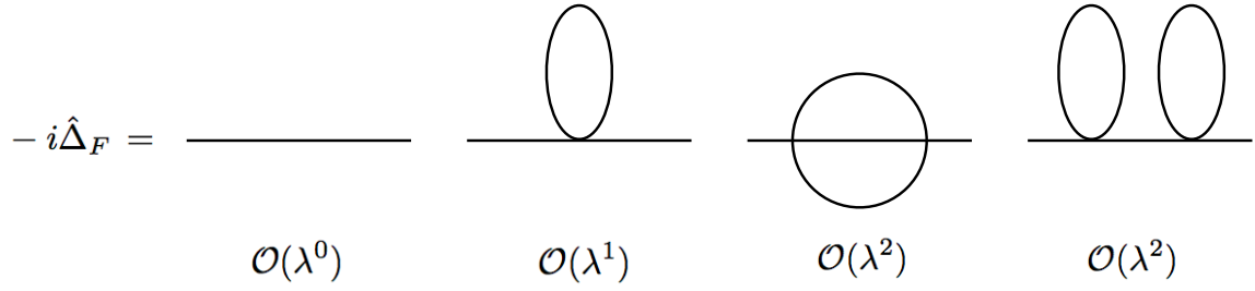
Figure 6. Some of the the Feynman diagrams that contribute to the calculation of the propagator \Delta_F in the interacting \lambda\phi^4 theory up to \mathcal{O}(\lambda^2) .
